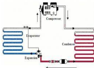
Gambar.3. skema air conditioner
