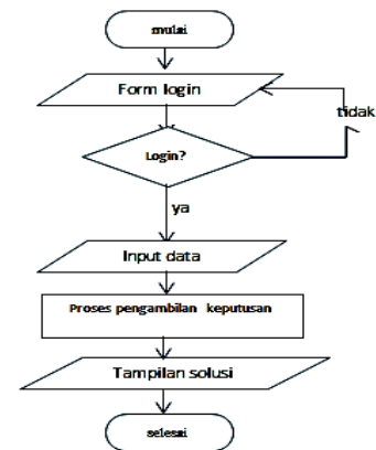
Gambar 6. flowchart user
